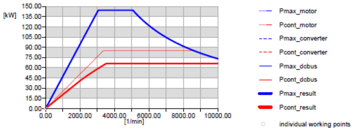
speed - power diagram
